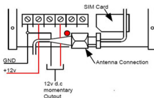
Connection Detail
